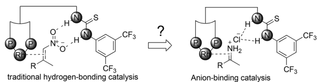
Figure 2. Extension of our rhodium/bis(phosphine) thiourea catalytic system.
